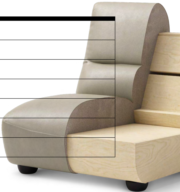
Snug Plus chair with arm 1SGPL1-900 (with left arm) 1SGPR1-900 (with right arm) 890H | 1040W | 1060D (mm) Seat width: 625mm Seat height: 425mm
